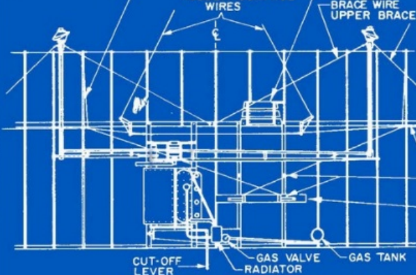
CENTER SECTION LOWER WING (FABRIC REMOVED)
